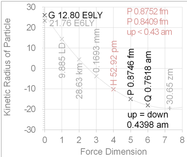
Fig. 7 Radius of proton and quark in kinetic state
