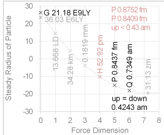
Fig. 8 Radius of proton and quark in steady state
