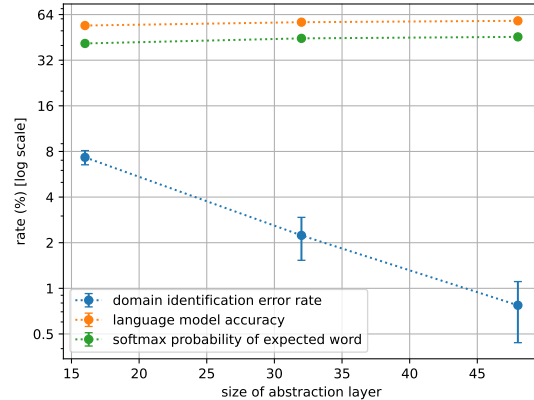
Figure 2: Model evaluation
