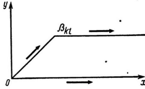
Pic.1. Contour [0, \beta_{k,l}] in complex plane \mathbb{C} .
