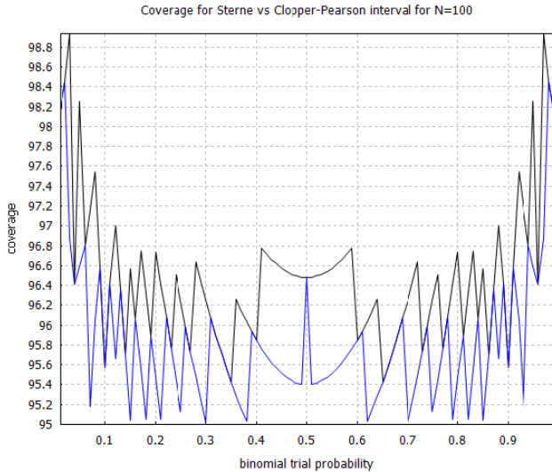
FIG. 2: Comparison of the coverage probability for the Clopper-Pearson interval [75] versus the Sterne interval [71] with sample size N = 100 . The black curve shows the coverage probability for the Clopper Pearson interval, and the blue curve, which is situated below the black curve, shows the coverage probability for the Sterne interval. The coverage probabilities were calculated using 0.01 increments on the horizontal axis.
