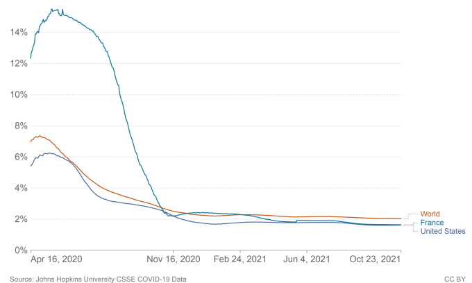
FIG. 10: Cumulative case fatality rate in the United States and France between April 2020 and November 2021.
