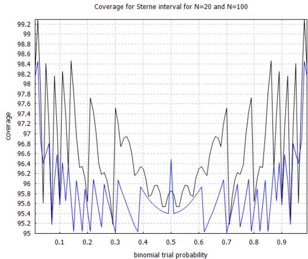
FIG. 1: Coverage probability for the Sterne interval [71] with sample sizes N = 20 and N = 100 . The black curve corresponds to N = 20 and the blue curve, which is situated below the black curve, corresponds to N = 100 . The coverage probabilities were calculated using 0.01 increments.
