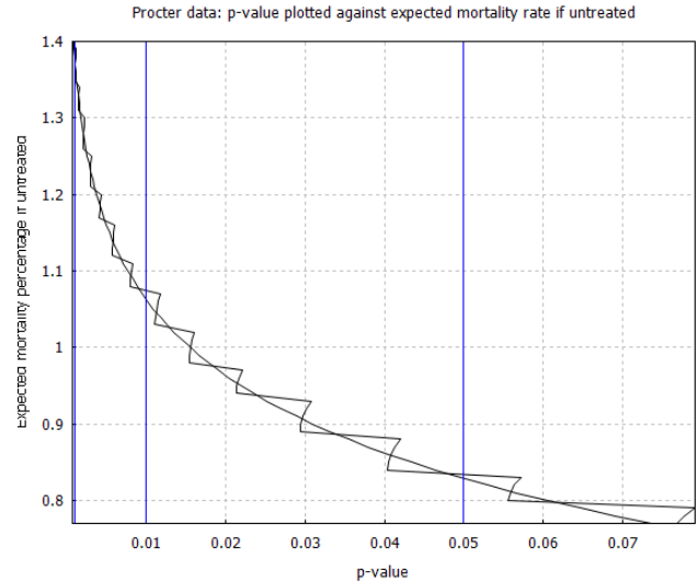
FIG. 3: Relationship between p -value and expected mortality rate for high risk patients without early treatment, based on the case series data from Procter's dataset of 869 high-risk patients [19]. The zigzag curve follows p(N, a, x) given by Eq. (2), whereas the smooth curve approximates the right tail terms in the p -value sum by replacing them with the left-tail terms on the horizontal axis.
