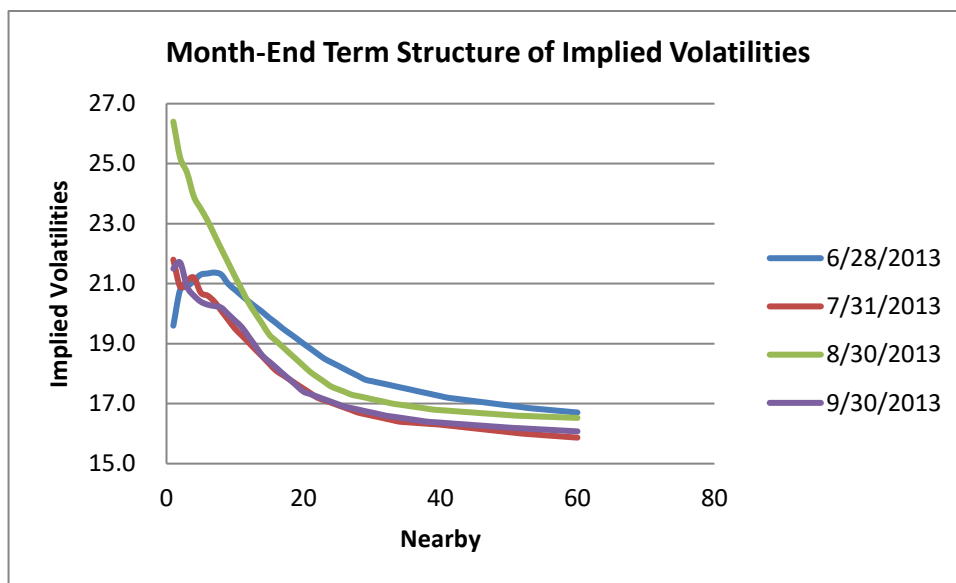
Figure 5. Month-end term structure of implied volatilities.
