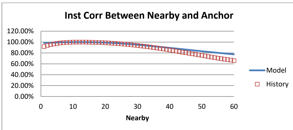
FIGURE 3 illustrates the correlation between different futures for West Texas Intermediate (WTI). More specifically, the graph plots the instantaneous correlation of the nearby number in the x-axis and the 12 th nearby.
