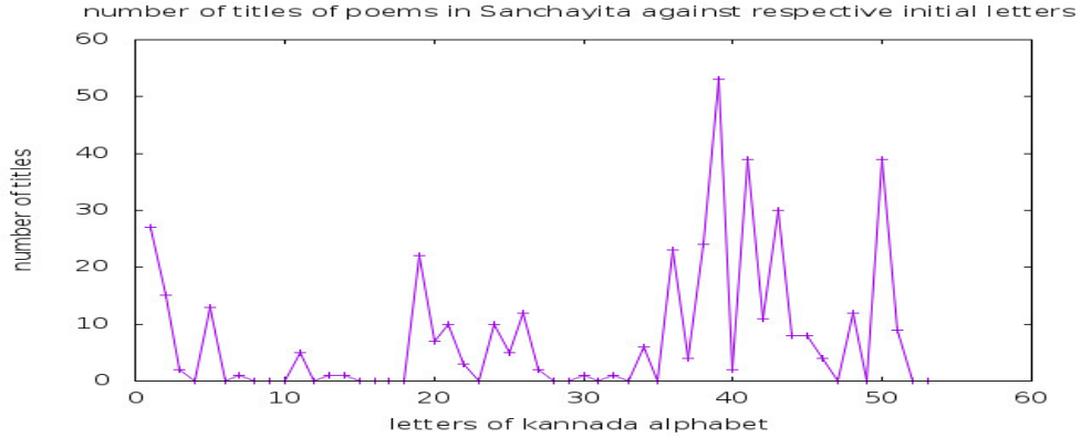
FIG. 1. The vertical axis is the number of the titles of the poems in the Sanchayita, [1]. The horizontal axis is the letters of the Bengali alphabet embedded in the Kannada alphabet. Letters are represented by the sequence number in the alphabet as it appears in the dictionary, [2].
