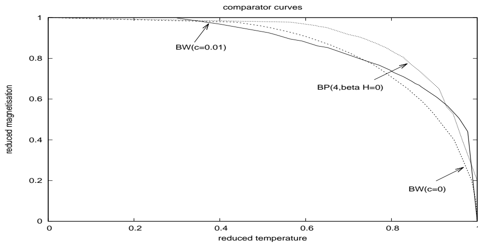
FIG. 3. Reduced magnetisation vs reduced temperature curves for the Bragg-Williams approximation, in the absence(broken line) of, BW(c=0) and the presence(inner in the top) of, BW(c=0.01), the external magnetic field, c = \frac{H}{\gamma\epsilon} = 0.01 , and the Bethe-Peierls approximation in the absence of external magnetic field, for four nearest neighbours (outer in the top).
