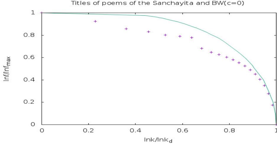
FIG. 4. The vertical axis is \frac{\ln f}{\ln f_{max}} and the horizontal axis is \frac{\ln k}{\ln k_{lim}} . The + points represent the titles of the poems of the Sanchayita, with the fit curve being the Bragg-Williams curve in the absence of external magnetic field, c = \frac{H}{\gamma\epsilon} = 0 .
