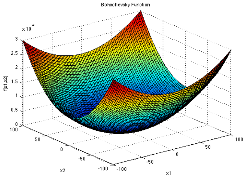
Figure 4. Bohachevsky Function
