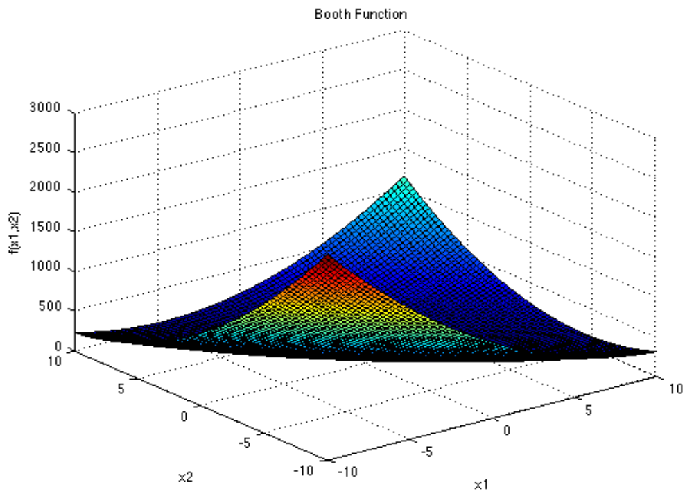
Figure 5. Booth Function
