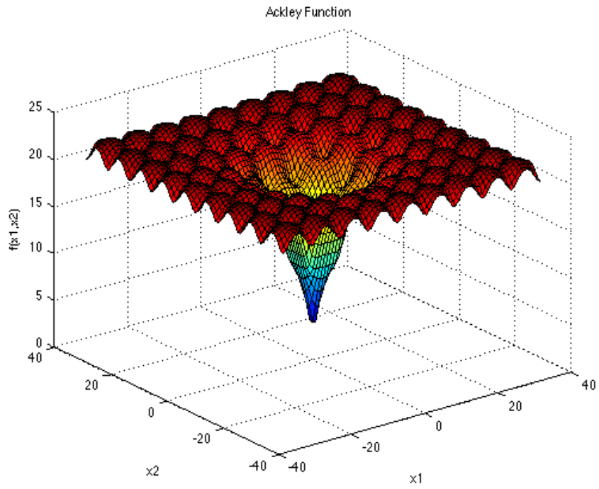
Figure 2. Ackley Function
