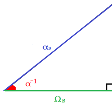
Figure 21. Geometric representation of the the density parameter for the baryonic matter
