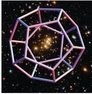
Figure 26. The shape of the universe is Poincaré dodecahedral space.
