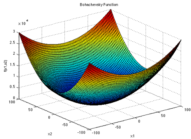
Fig. 4. Bohachevsky function
