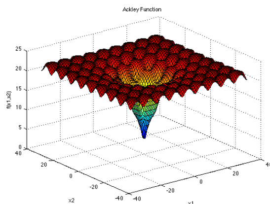
Fig. 2. Ackley function
