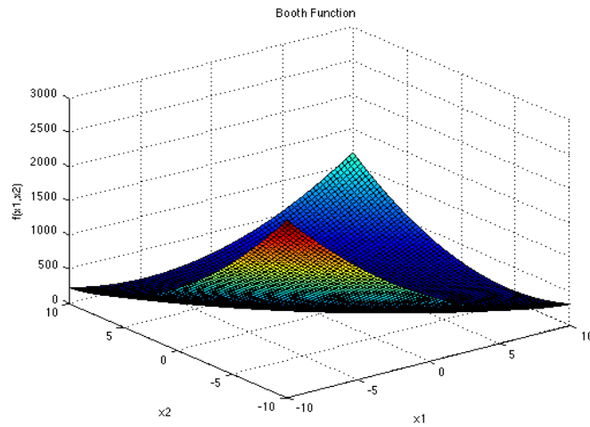
Fig. 5. Booth function
