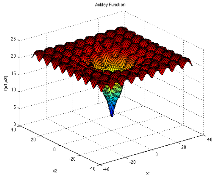
Fig. 2. Ackley function
