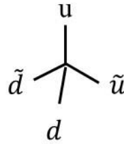
Right chiral
