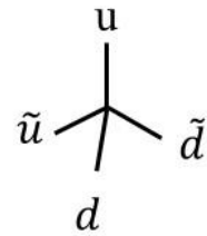
QCD tetrahedron
