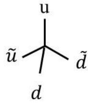
Left chiral
