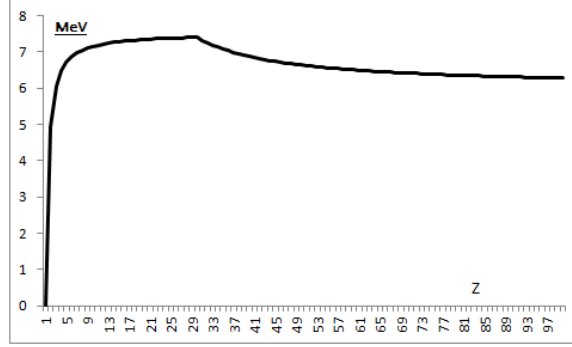
FIGURE 3. Average Binding Mass: \bar{M}(0) - \bar{M}(Z)
