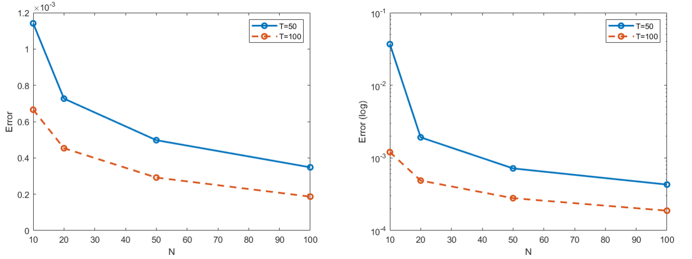
Figure 4: Mean absolute error (MAE) for the estimation of the true mean of the posterior with different number of particles by ATAIS. (Left: location example. Right: multi-output example with the scale for y-axis in logarithm).
