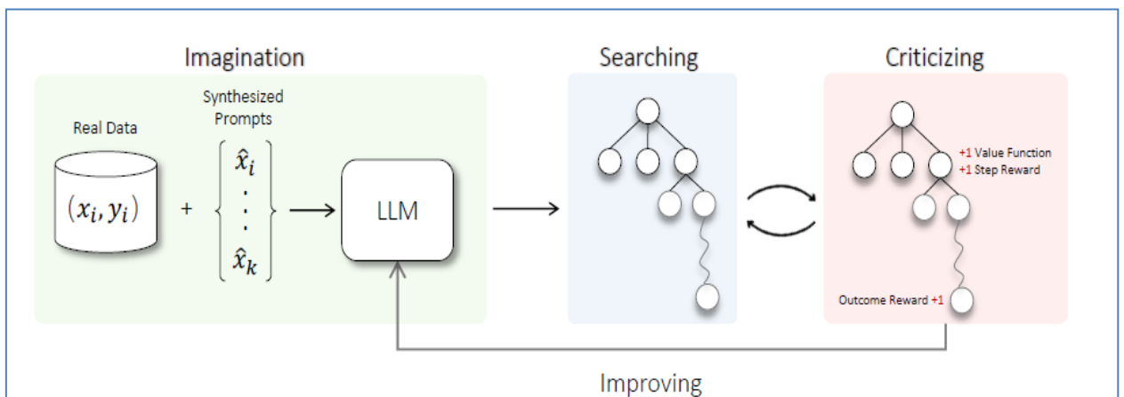
Figure 1: Imagination-Searching-Criticizing self-improvement loop: Imagination component synthesizes prompts as new learning examples, with MCTS searching better trajectories guided by signals from critics for policy improving.
