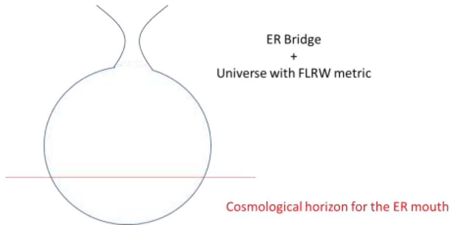
Figure 2: A geometry à la Wheeler’s bag of gold per [38,39]. The expanding universe (~FLRW [170]) is often call baby universe. Our analysis further calls for matter, gravity (and entanglement) to be captured behind the apparent cosmological horizon of the FLRW expanding baby universe, with respect to the mouth of the ER wormhole as hinted in red. A conventional Wheeler’s bag of gold as in [38,39], and the mechanisms invoked in [37], do not rely, to the best of our understanding, on the apparent cosmological horizon, but they should.
