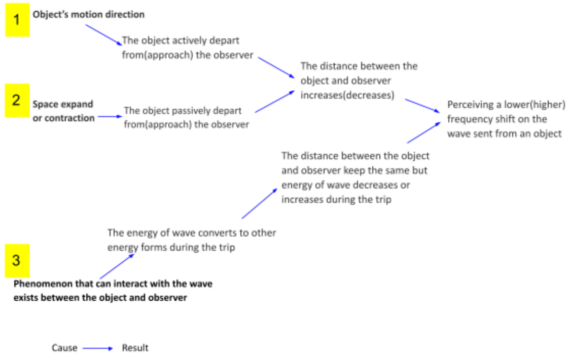
Fig. 3. All possible causes for perceiving a frequency shift of wave sent from an object
