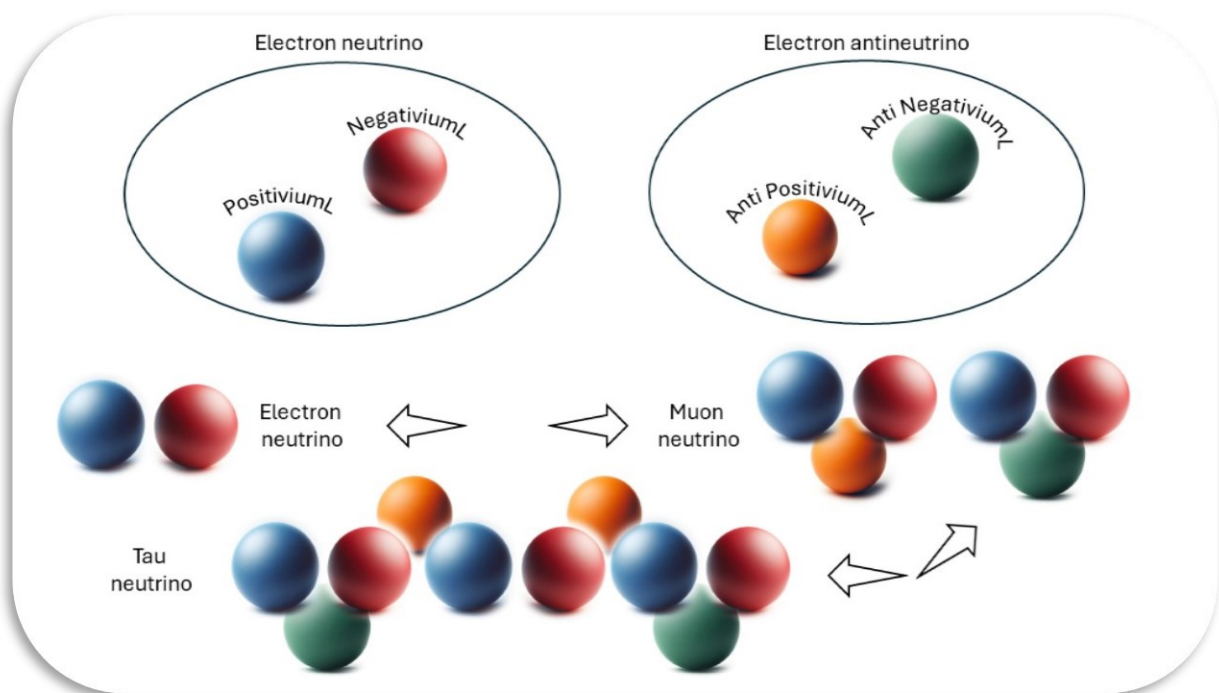
Figure 1 Neutrinos oscillations
