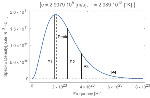
Figure 2. The Black Body spectrum is the mixed quarks and gluons sea in the quiescent proton. The intensity and spectral energy density on the vertical axis. The dashed vertical line is the peak, and the peak frequency is 5.8802 \times 10^{10} \times 2.989^{12} = 1.758 \times 10^{23} Hz .
