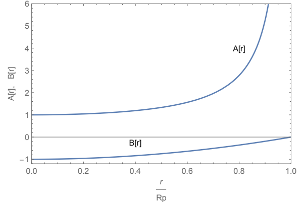
Figure 1. The metric tensor of the proton-space is flat at the proton's center and has a singular surface at the radius in the metric space component, the time metric components becomes zero at proton surface. Objects inside this proton space are confined due to the singular surface and can not escape; quarks and gluons live in their own universe, until disturbed by high energy collisions.
