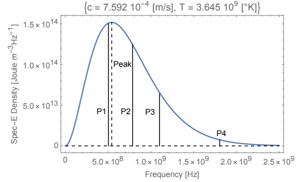
Figure 5. The Black Body spectrum of the mixed quarks and gluons in the quiescent proton. The intensity, and spectral energy density on the vertical axis. The dashed vertical line is the peak, and the peak frequency is 5.8802 \times 10^{10} \times 1.67 \times 10^9 = 5.4253 \times 10^8 .
