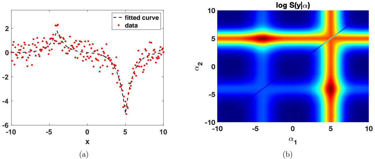
Figure 1: (a) One realization of the data vector \mathbf{y} and a corresponding fitted curve according to the observation model. (b) Example of the log area under the likelihood \log S(\mathbf{y}|\boldsymbol{\alpha}) in one realization of the data vector \mathbf{y} . We can see that the maxima are localized around approximately [-4, 5] and [5, -4] (just [-4, 5] is admissible since \alpha_1 < \alpha_2 ).
