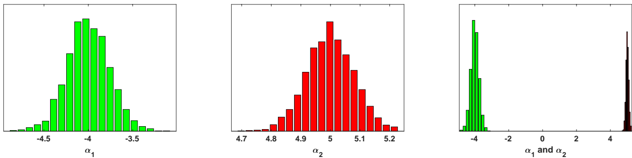
Figure 2: Histograms of each component of estimated vector \boldsymbol{\alpha} = [\alpha_1, \alpha_2]^\top (maximizing S(\mathbf{y}|\boldsymbol{\alpha}) ) over 2000 independent realizations. We can observe that bias is virtually zero and the variance is bigger for \alpha_1 with respect to \alpha_2 . This is reasonable looking the realization of data in Figure 1(a) where the (negative) pick at x = 5 seems much more clear/evident, than the first pick at x = -4 .
