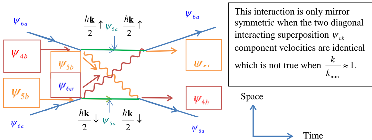
Figure 10.1 Covariant interaction (as in Eq. (3.3.4) and the top half of Figure 3.3.3) between fermion (subscript a) and photons (subscript b and in boxes) eigenfunctions. Orange and magenta are used for bosons, blue and green for spin 1/2 to help identify the transitions at each of the four spacetime corners. This is one process, but a superposition of two diagonal components splitting the 3 momentum \hbar\mathbf{k} equally.
