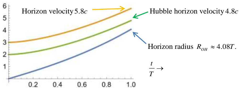
Figure 8.2.6 A plot of the horizon velocity \dot{R}(t) , the Hubble horizon velocity \dot{R}(t) - 1 , and the horizon radius R(t) , all with d = 1.2 .
