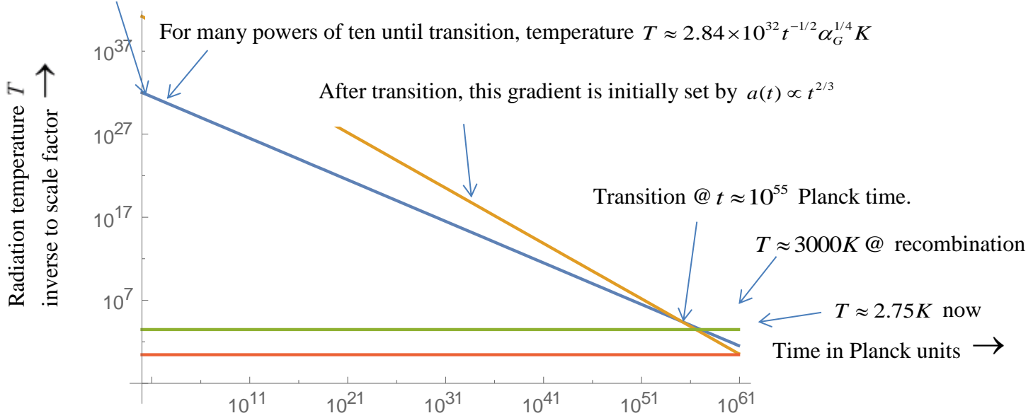
Figure 5.3.2 A logarithmic temperature plot with \alpha_G \approx 0.2 from t \approx 2 Planck time,
