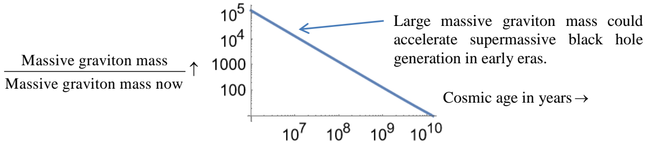
Figure 8.2.1 A logarithmic plot of the increase in massive graviton mass versus cosmic time. One of the implications of this early larger massive graviton mass is that the average size of galaxies is proportional to the massive graviton Compton wavelength which is \propto k_{\min}^{-1} . Equation (8.2.2) is r_{Halo} \propto k_{\min}^{-1} , which is also approximately inverse to Cosmic time, as has been recently observed by the James Webb telescope.
