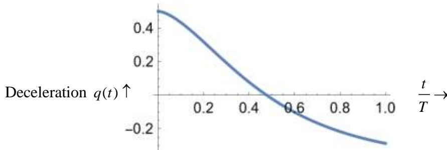
Figure 8.2.2 Deceleration as a function of cosmic time with d = 1.2 in Eq.(8.2.19).
