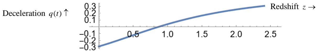
Figure 8.2.4 A plot of deceleration versus redshift, with z_t \approx 0.87 at transition.
