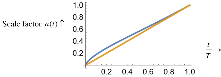
Figure 8.2.3 A plot of the scale factor with d = 1.2 showing that it starts at a(t) \approx \propto t^{2/3} and is now approximately a(t) \approx \propto t as in conventional cosmology.
