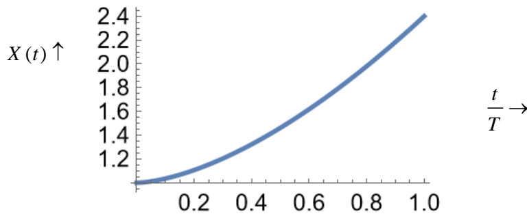
Figure 8.2.5 A plot of X(t) with d = 1.2 .
