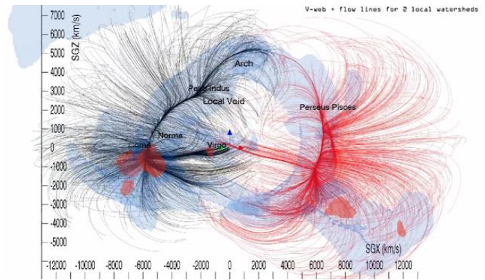
Figure 2. A representation of structure and flows due to mass within 6,000 \text{ km s}^{-1} ( \sim 80 \text{ Mpc} ).
