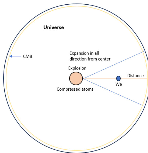
Fig: Representation of the Universe
