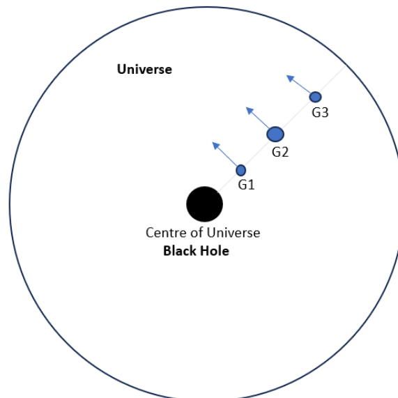
Fig: The figure showing that, why universe looks like it expanding ?
