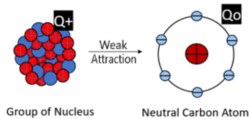
Fig 3. This figure showing the interaction of a group of nuclei with a neutral atom.
