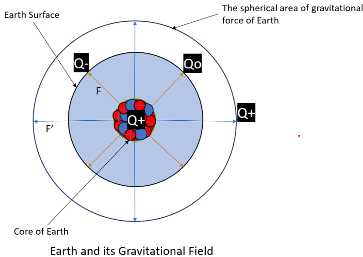
Fig 4. This figure demonstrates the location of nuclei present in the core of the Earth and explains how Earth's gravitational force operates.
