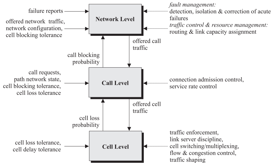
Figure 1: Multilevel traffic control in ATM networks.
