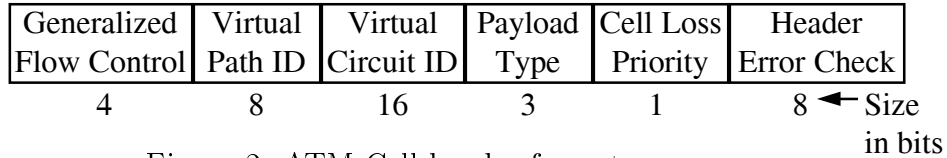
Figure 2: ATM Cell header format
