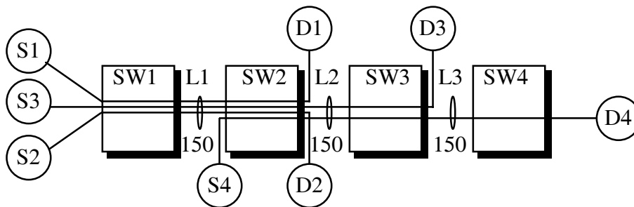
Figure 3: Sample configuration for max-min fairness
