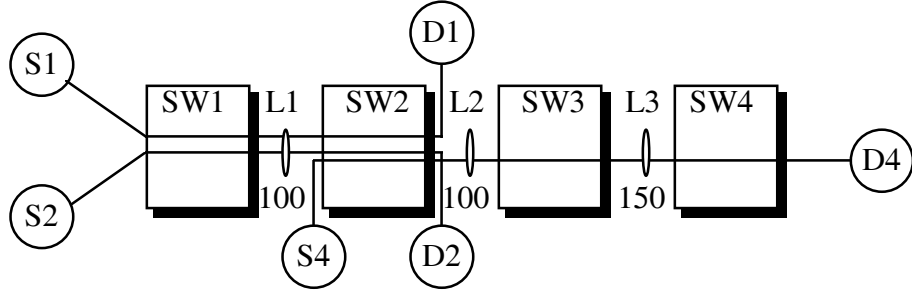
Figure 4: Configuration after removing VC 3.
