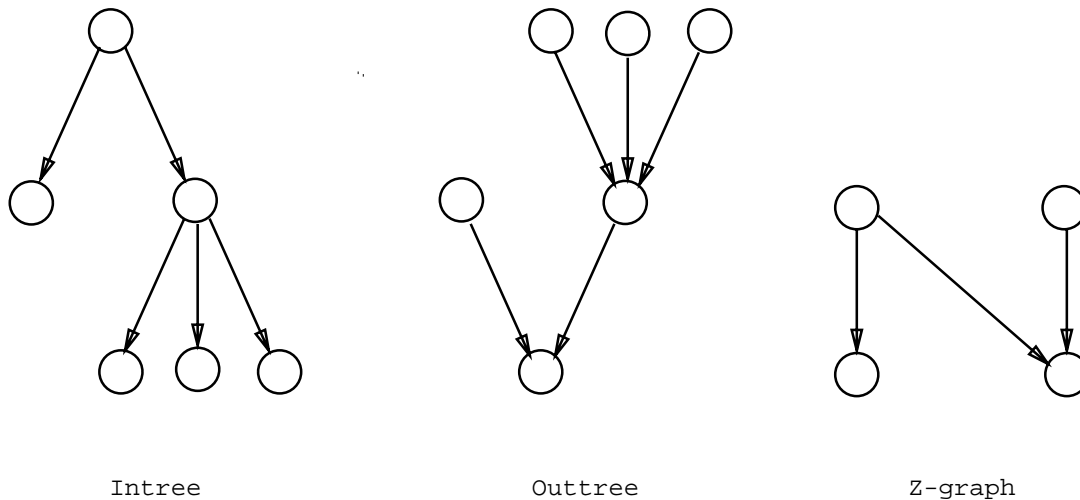
Figure 2: Precedence Relations
