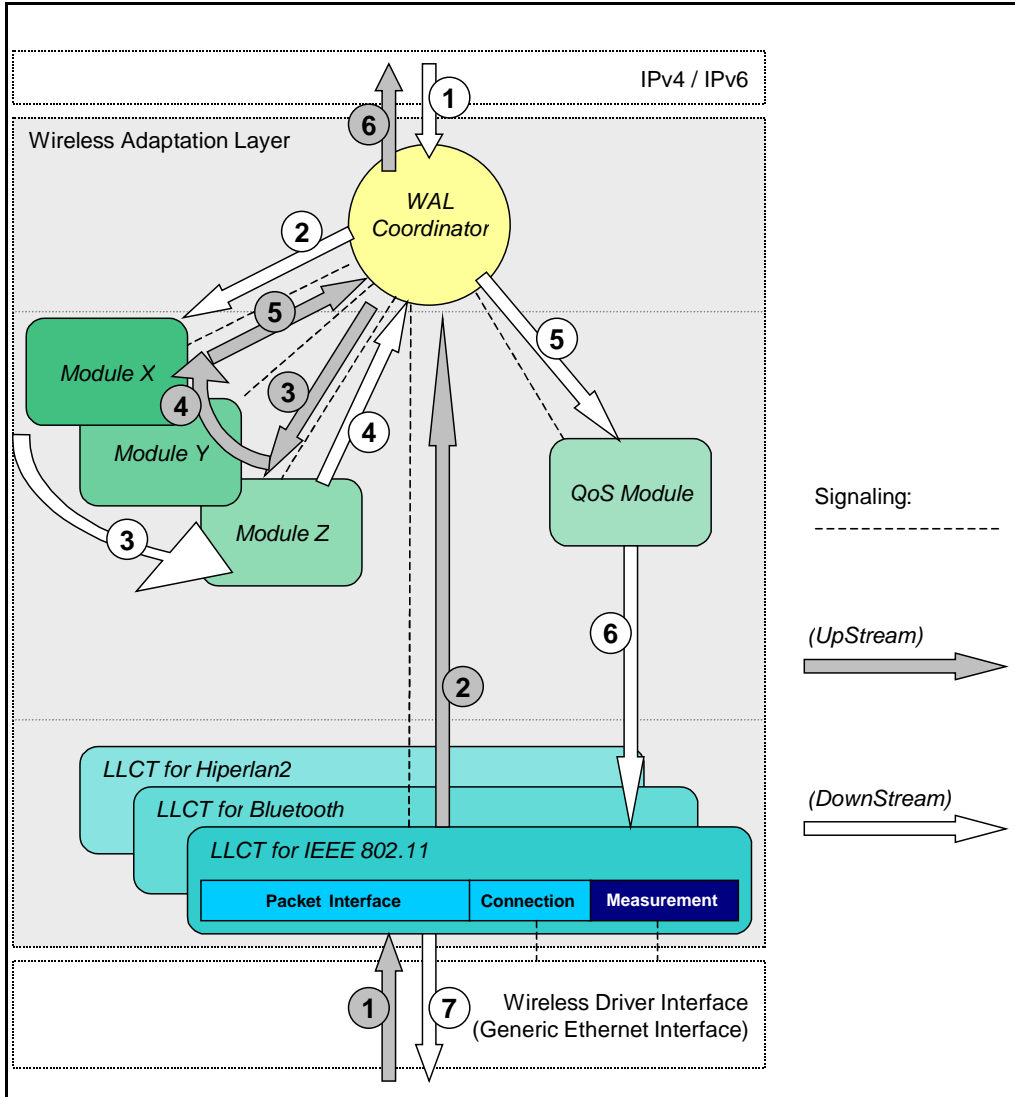
Figure 5. The WAL Architecture
