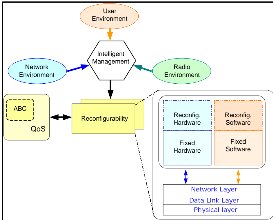
Figure 3. Essential elements of reconfigurability involved in the communication layers for ABC.
