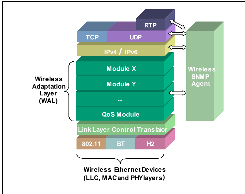
Figure 4. The Wireless Adaptation Layer
