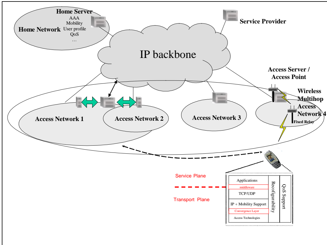
Figure 2. ABC reference system architecture
