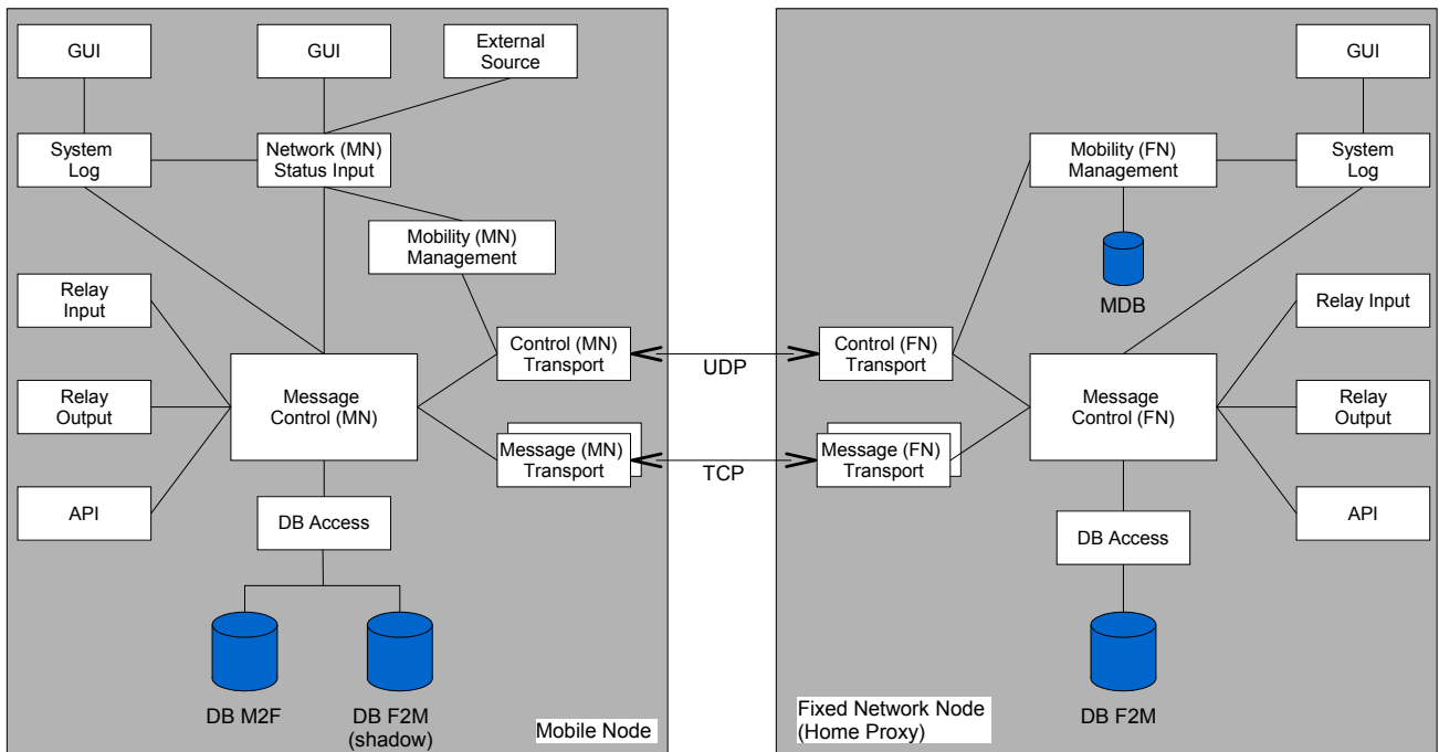
Fig. 6. Building blocks of the middleware component
