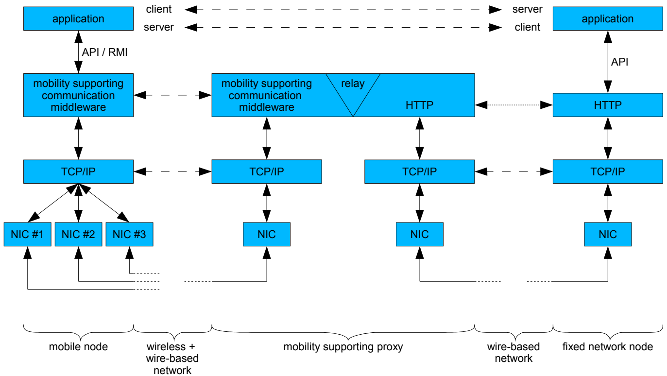
Fig. 5. Protocol stack view of the system architecture for the HTTP case
