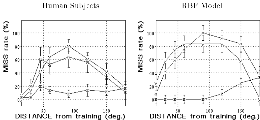
Figure 9: Left : human performance in the recognition of rotated wire-like 3D objects (Bülthoff and Edelman, 1992). Error rate of subjects trained on single view is plotted vs. distance between training and test views. Note poor generalization across rotations in depth (curves marked by x, y ), compared to rotation in the image plane (curve marked by z ; see text). Right : performance of the HyperBF network model (Poggio and Edelman, 1990; Edelman and Poggio, 1992; Bülthoff and Edelman, 1992) in the same task.
