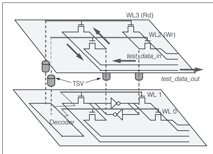
Figure 4. 3D memory port-splitting (four ports, two for each die layer). (WL: word line.)
