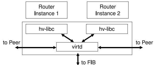
Figure 2: Implementation architecture.
