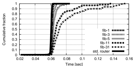
Figure 7: BTR pass-through time.
