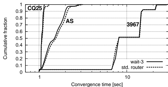
Figure 8: Network-wide simulations, per-router convergence delay distribution.
