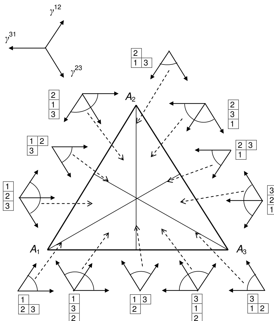
Figure 1. Compartments C_\sigma , corresponding cones Q_\sigma (the angles) and all tableaux \sigma for the Markov chain with three states (the choice of equilibrium (p_i^* = 1/3) , does not affect combinatorics and topology of tableaux, compartments and cones).
