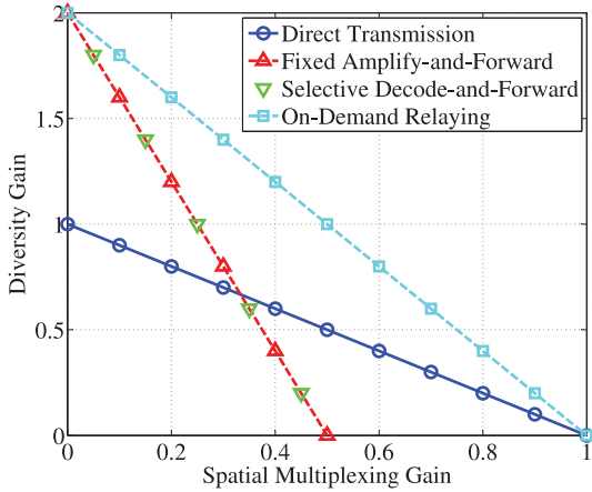
Fig. 2. DMT curves of a direct transmission and three cooperative transmission schemes involving one relay terminal: fixed amplify-and-forward, selective decode-and-forward, and on-demand relaying [7].
