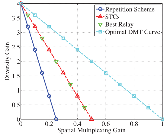
Fig. 3. DMT curves of three cooperative transmission schemes with N relay terminals ( N = 4 ): fixed AF protocol using a repetition scheme at the relay terminals (Repetition Scheme) [7], the fixed AF protocol implementing STCs (STCs) [3], and the AF protocol based on the selection of the best relay terminal (Best Relay) [9], and the optimal DMT curve (Optimal DMT Curve) [10], [11].
