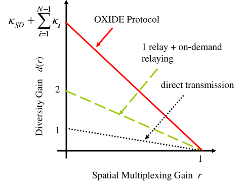
Fig. 9. DMT curve of three protocols : the OXIDE protocol, the direct transmission, and the on-demand cooperation with one relay terminal [7]. For the special case of Rayleigh fading, \kappa_{SD} + \sum_{i=1}^{N-1} \kappa_i = N .
