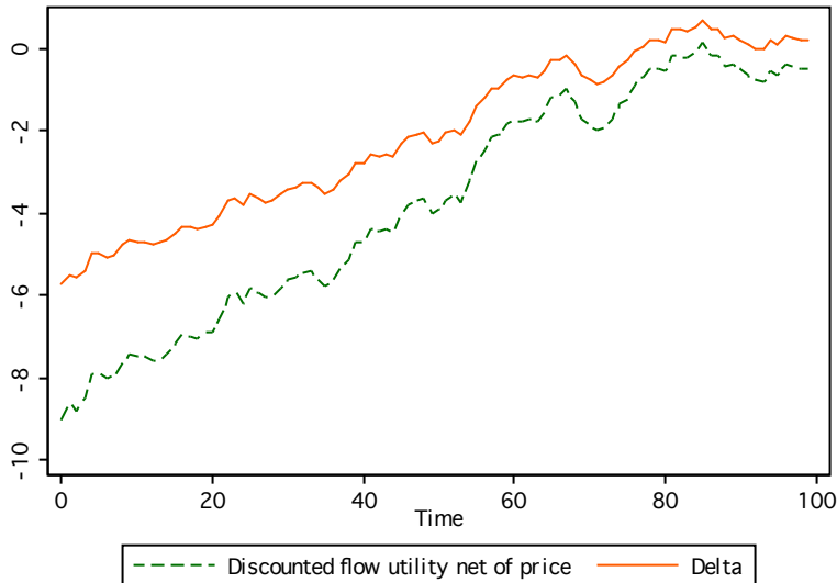
Figure 1: Simulated evolution of flow utility and delta in a simple example
