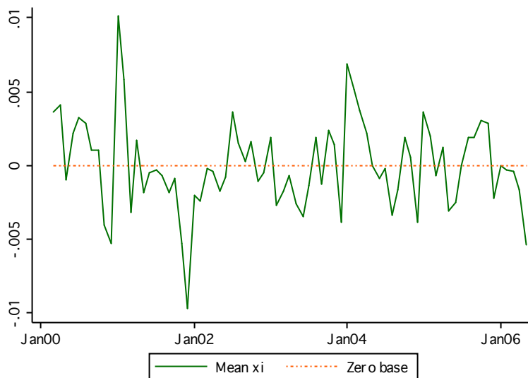
Figure 9: Average estimation error ( \xi_{jt} ) by month
