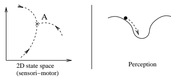
Fig. 1. Trajectories converging towards a fixed-point attractor A and the corresponding potential function (in 1D only)
