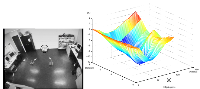
Fig. 8. left: Top view of 2 robot positions and associated actions during learning phase. right: Final Perception function
