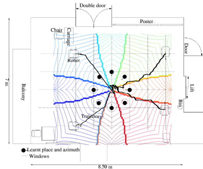
Fig. 5. Top view of an indoor environment with superposed theoretical place fields and homing trajectories for four initial robot positions. 8 places (black circles) were first learned at 1 m from the goal.
