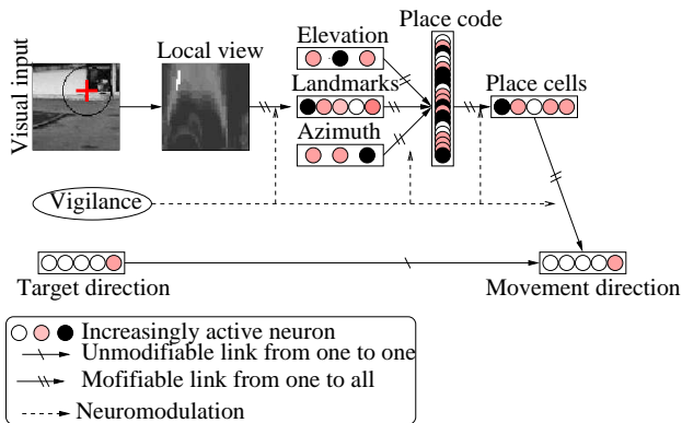
Fig. 4. PerAc architecture for a homing task. The Target direction and Movement direction are competitive groups.
