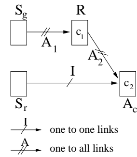
Fig. 2. A neuronal sensorimotor architecture PerAc from [6]. S_r , S_g , R , Ac are neurons vector representing the 2 sensation inputs, the learned categories and the possible output actions. A_1 , A_2 , I are connection weights matrixes and c_1 , c_2 represent operators associated to group of neurons.
