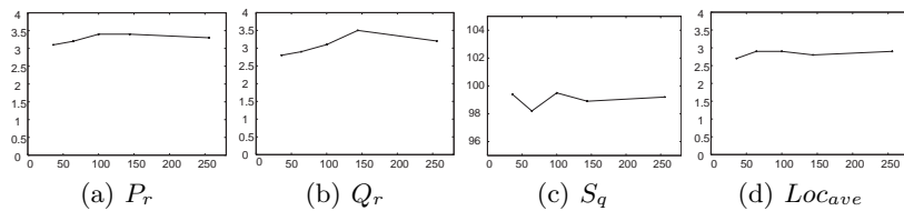
Fig. 4. Scalability of HTL in mobile networks
