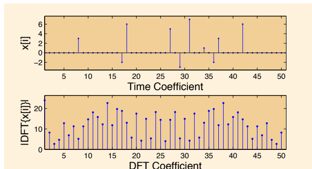
Fig. 1. Sparse discrete time signal with its Discrete Fourier Transform (DFT).
