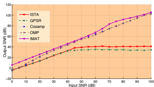
Fig. 5. Performance comparison of some reconstruction techniques for DFT sparse signals.
