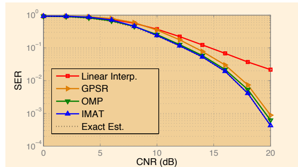
Fig. 28. SER (Symbol Error Rate) vs. CNR (Carrier to Noise Ratio) for the ideal channel, linear interpolation, GPSR, OMP and the IMAT for the Brazil channel at Fd = 0 without zero-padding effect.
