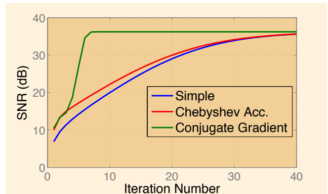
Fig. 8. SNR improvement vs. the no. of iterations for a random sampling set at the Nyquist rate (OSR=1) for a bandpass signal.
