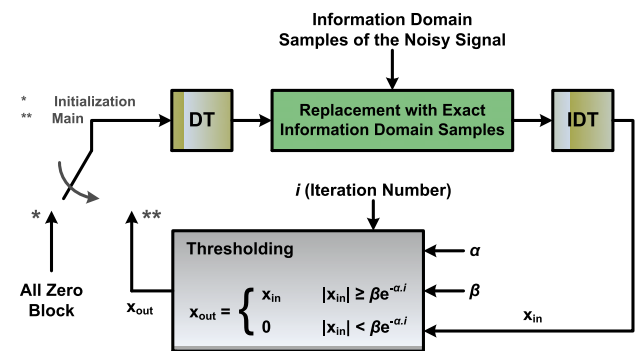
Fig. 9. The IMAT for detecting the number, location, and values of sparsity.
