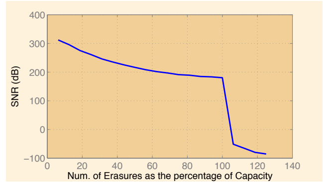
Fig. 13. Recovery of a burst of 16 sample losses.
