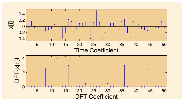
Fig. 2. Sparsity is manifested in the frequency domain.
