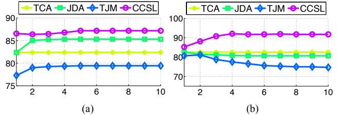
Figure 4: Convergence analysis (accuracy (%) vs. number of iterations) on (a) balanced domain pair of A \rightarrow C and (b) imbalanced domain pair of A \rightarrow C_5 .
