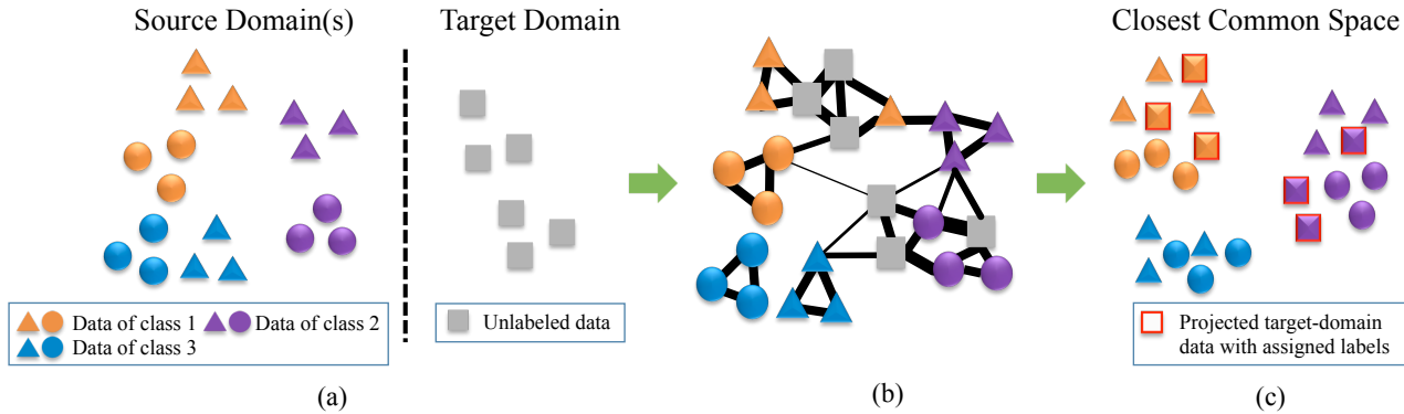
Figure 1: Overview of our approach: (a) Source and target-domain data, (b) exploiting label and latent-domain information within and across domains, and (c) the resulting space for adaptation and classification. Note that different shapes correspond to different domains/datasets, while the colors denote the object categories.
