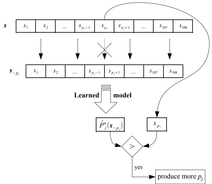
Fig. 3. Agent production behavior
