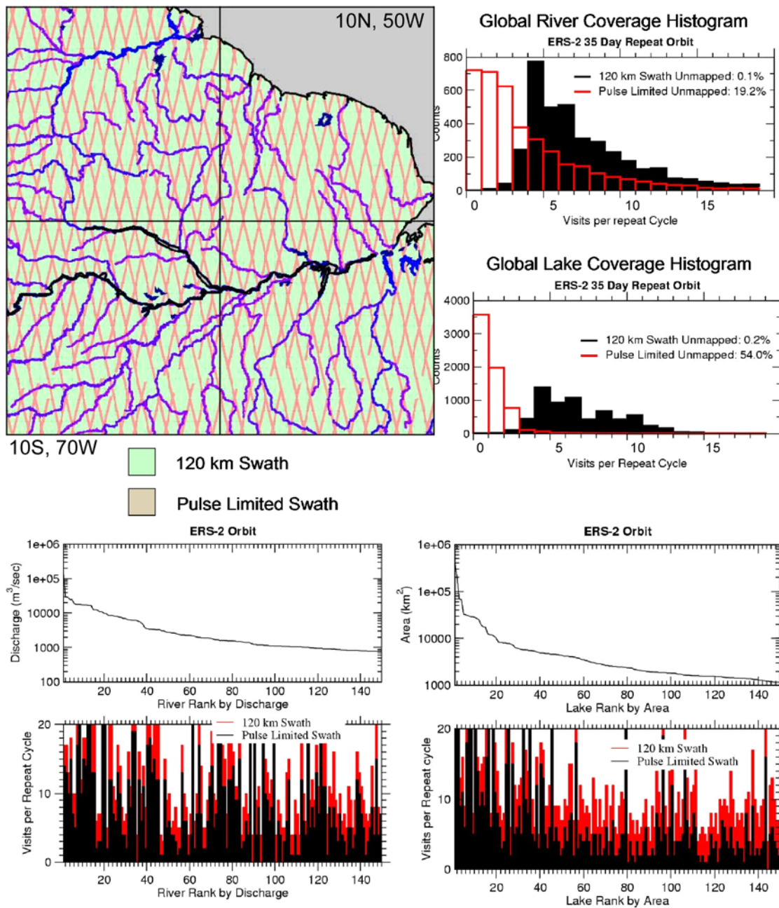
Figure 14. Global lake and river coverage study using the 35-day repeat cycle of ERS (~98° inclination and Sun-synchronous). Comparisons between profiling and imaging technologies demonstrate that 19% of the rivers and 54% of the world’s lakes are missed by a profiling instrument, whereas far less than 1% of rivers and lakes are missed by an imager. As indicated in the bottom four plots, profiling technologies miss altogether five and one of the world’s top 150 rivers and lakes, respectively (largest missed discharge is nearly 5000 m 3 /s; largest missed area is ~300 km 2 ), whereas imagers provide complete coverage.
