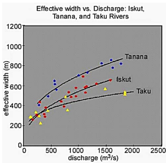
Figure 10. In situ discharge correlated with remotely sensed inundated area. “Effective width” determined from SAR imagery is a measure of the inundated area during flood events for three braided rivers in the Arctic. Discharge was determined from a gauge at a downstream coalescing of channels. The three curves represent possible rating curves to predict discharge in the absence of gauge data [Smith et al. , 1996].
