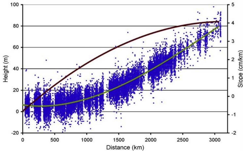
Figure 9. Estimated elevation (green line) and slope (red line) of the Amazon River. A third-order polynomial (green line) fitted to water surface SRTM elevations (blue dots) from the main Amazon channel provides a derivative for estimating slope variations along the entire profile [LeFavour and Alsdorf, 2005].
