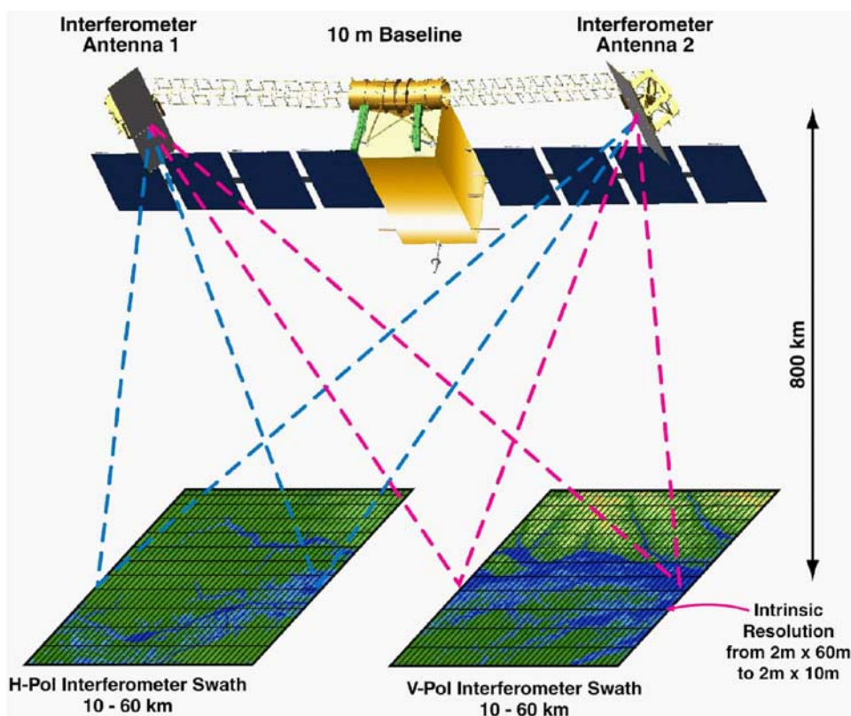
Figure 15. Conceptual view of KaRIN, the Ka Band Radar Interferometer, an interferometric altimeter. Maximum incidence angle is 4.3^\circ ; thus the instrument operates very near nadir where water surfaces yield strong radar returns. At Ka band the interferometer will penetrate clouds and relies on subtle canopy openings to penetrate to any underlying water surfaces (openings of only 20% are sufficient). Spatial sampling resolutions are noted in Figure 15. Height accuracies will be \pm 50 cm for individual “pixels”; thus centimetric accuracies are achieved through polynomial averaging methods.
