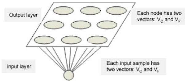
Figure 3. The basic principle of ConSOM.
