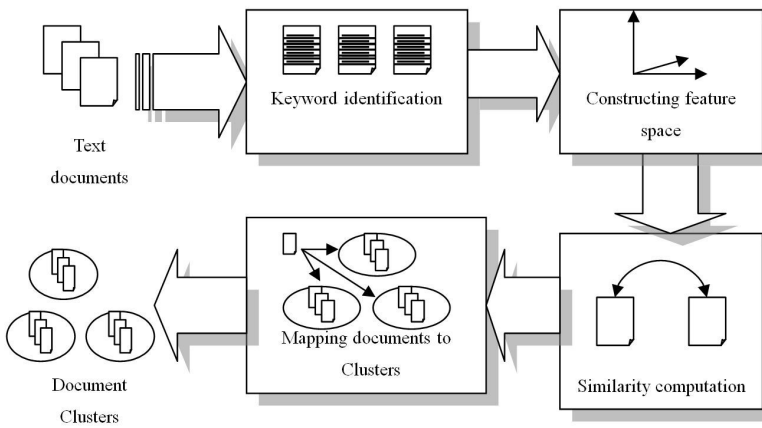
Figure 1. The main framework for text clustering system.
