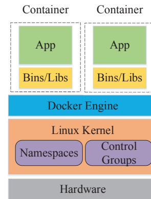
Fig. 5: Architectural Overview of the Docker Container
