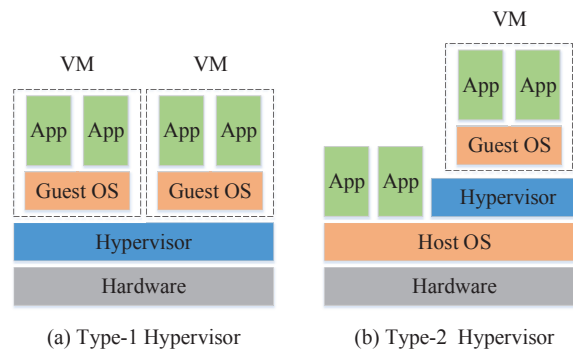
Fig. 3: Hypervisor
