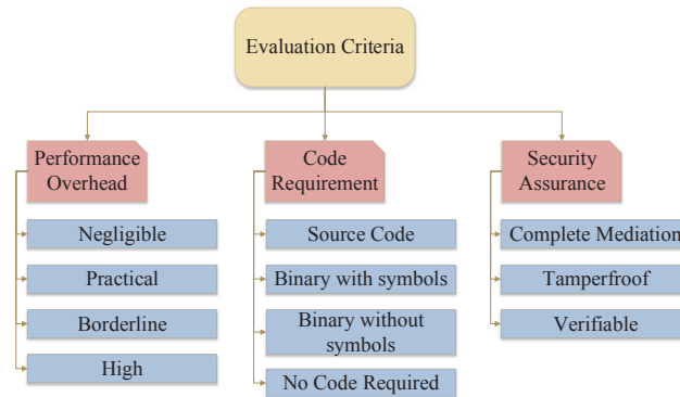
Fig. 2: Evaluation Criteria
