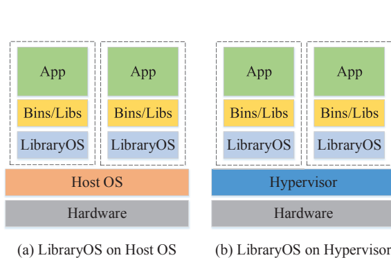
Fig. 4: LibraryOS
