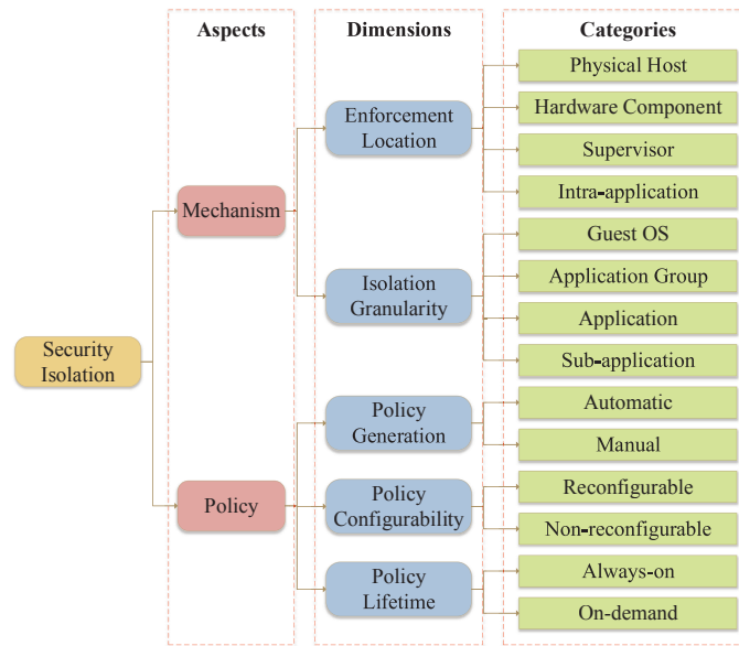
Fig. 1: Hierarchical classification structure for security isolation.
