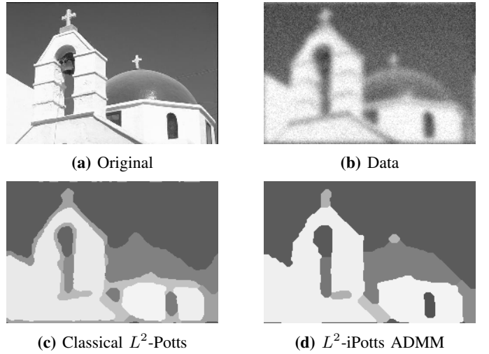
Fig. 4: Segmentation using the classical (9) and the inverse Potts functional (1) of a blurred and noisy natural image (size 241 \times 161 , image source [59]). Due to the blurring, the classical Potts segmentation exhibits additional segments at the boundaries, whereas segmentation with our inverse Potts ADMM detects sharp boundaries.
