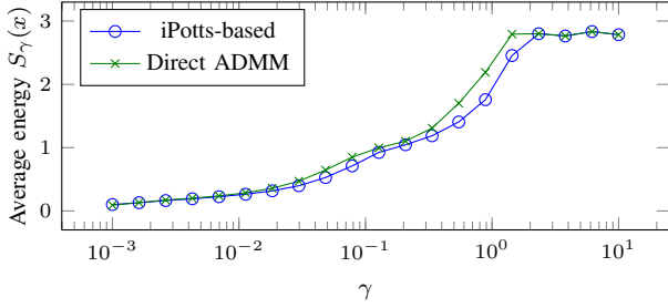
Fig. 8: Final total energy S_\gamma(x) of the sparsity problem using the iPotts based method (Algorithm 2) and the “direct” ADMM method (Subsection V-B) for different parameters \gamma . The iPotts-ADMM algorithm reaches lower energies over the whole parameter range. This indicates the superiority of the first method. Computed values are averages over 50 experiments.
