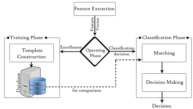
Fig 5. Training and classification phases
