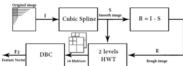
Fig 4. Rough – Smooth technique
