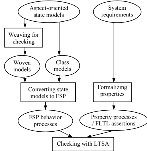
Figure 5. The model-checking process
