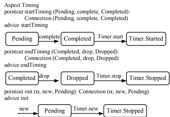
Figure 4. The Timing aspect model
