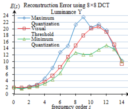
Figure 4. Average reconstruction error of an increment on DCT coefficient Luminance for 40 real colour image.
