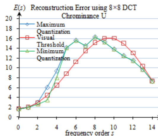
Figure 5. Average reconstruction error of an increment on DCT coefficient Chrominance for 40 real colour image.
