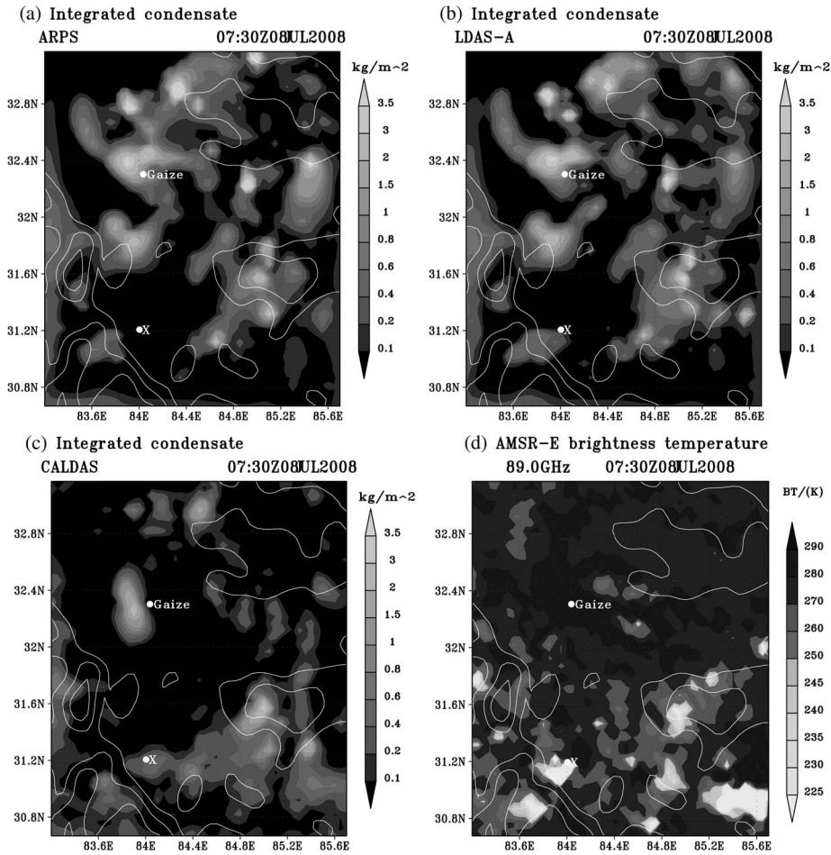
Fig. 5. Spatial distribution of vertically integrated condensate (liquid plus solid phases) ( \text{Kg}/\text{m}^2 ) at 0730 UTC on 08th July 2008; (a) ARPS, (b) LDAS-A, (c) CALDAS, and (d) AMSR-E brightness temperature at 89 GHz.
