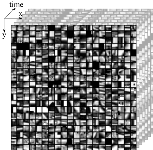
Figure 5: Over-complete dictionary is learned from 20 videos of resolution 384 \times 216 , rotated into 8 different orientations and played forward and backward. The frame rate of the training videos matches the target frame rate (300 – 1000 fps). The learned dictionary captures various local features and structures in videos, such as edges shifting in different orientations. Please see the project web-page [24] for videos of the learned dictionary.
