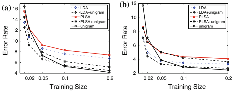
Fig. 5 Classification error rate versus training size. a Error rate versus training size on Reuters, b error rate versus training size on TDT2
