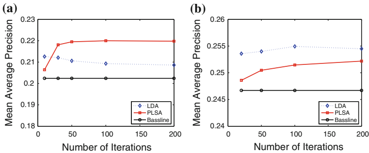
Fig. 11 MAP versus number of iterations. a SJMN: number of iterations, b LA: number of iterations.
