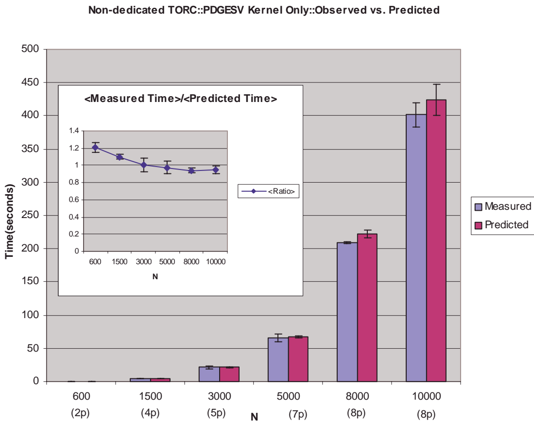
Figure 1: Performance Model vs. Measured Performance
