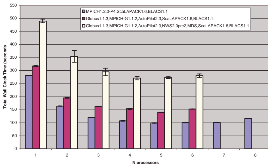
TORC::Software Comparison::Sample Run N=5000::Total Turnaround Time in Solving AX=B
