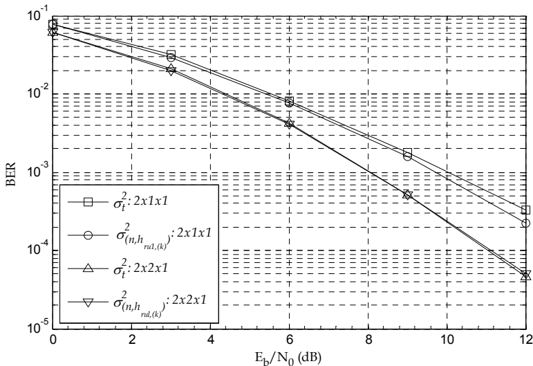
Fig. 10. System performance
