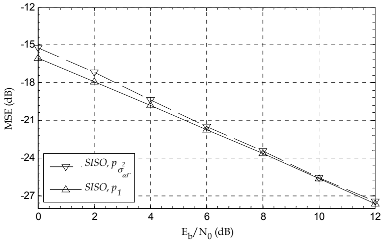
Fig. 7. Channel estimation MSE performance
