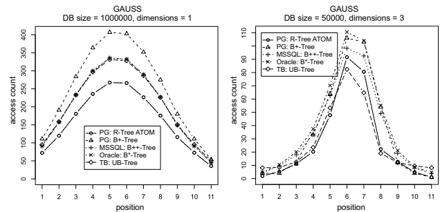
Figure 14: Moving window query
