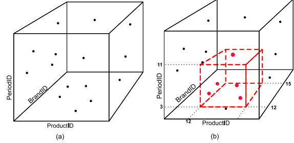
Figure 2: Multidimensional visualization of data (a) and window query (b)
