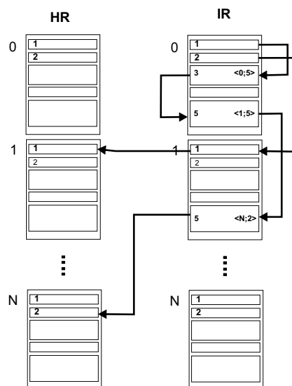
Figure 5: Chained IRs referring to HRs.
