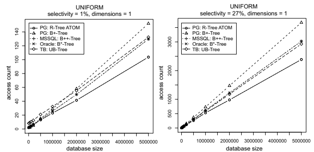
Figure 9: Impact of dataset size on access count (different query selectivities)
