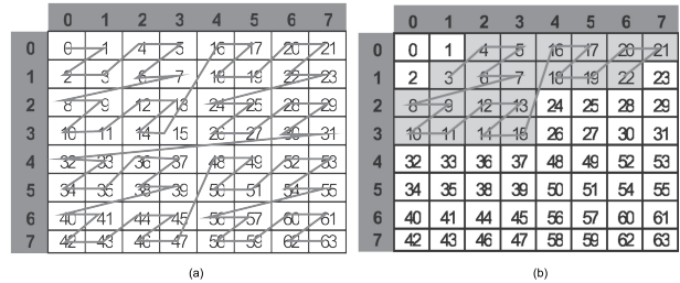
Figure 4: Z-curve (a) and Z-region (b).
