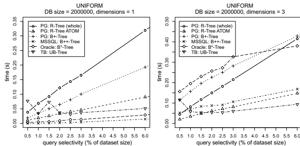
Figure 15: Impact of query selectivity on realtime
